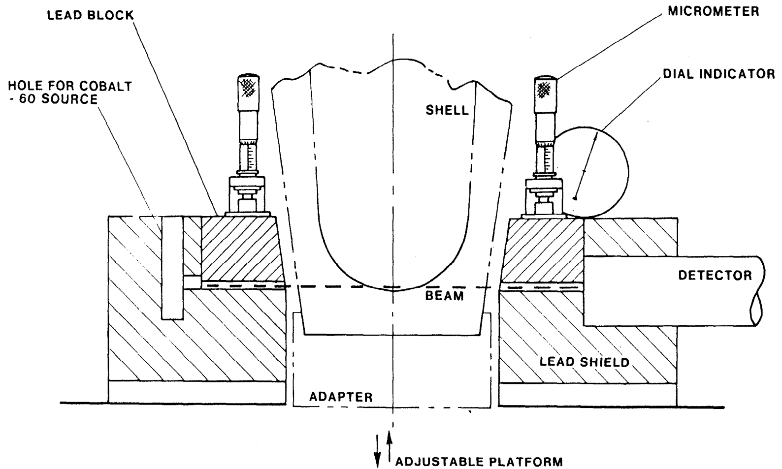
Fig 11 Sketch of \gamma -Ray Transmission Gauge for Base Separation Detector
